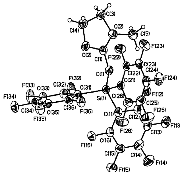
Figure 2. The molecular structure of 9 ; non-hydrogen atoms are shown as thermal ellipsoids at 50% probability; selected bond lengths (Å): Si(1)–O(1) 1.632(3), O(1)–C(1) 1.347(5), Si–C (average) 1.886(5); bond angles ( ^{\circ} ): Si(1)–O(1)–C(1), C–Si–C 110.14, O–Si–C 108.66
