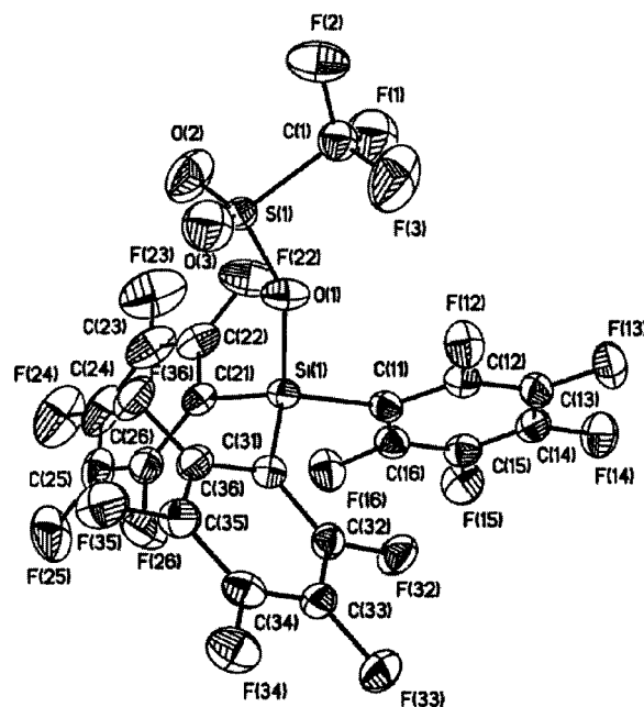
Figure 1. The molecular structure of TPFS triflate 1 ; atoms are shown as thermal ellipsoids at 50% probability; selected bond lengths (Å): Si(1)–O(1) 1.663(2), Si–C (average) 1.858(3), S–O(1) (average) 1.510(2), S–O 1.433(3); bond angles (°) Si–O–S (average) 149.5, O–Si–C (average) 106.8, C–Si–C 112.0
